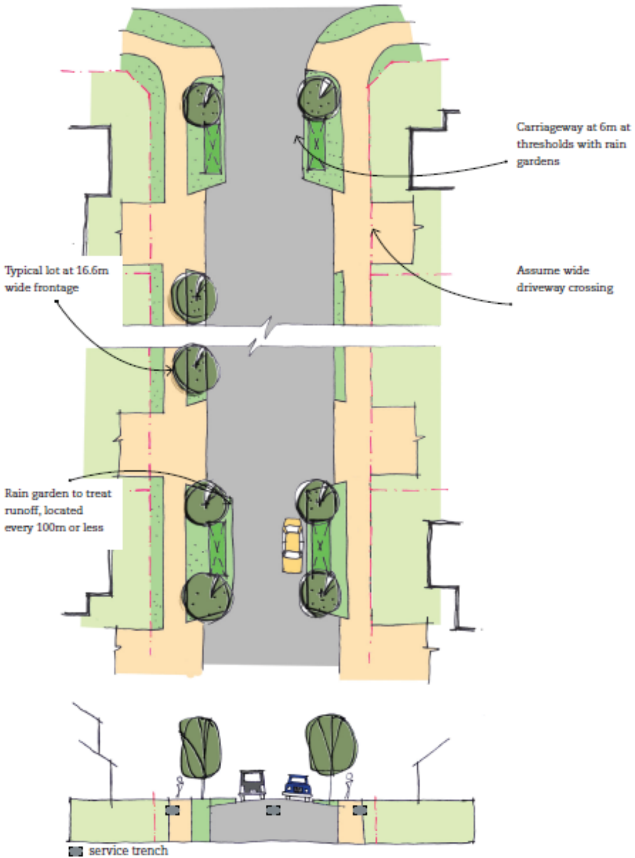
Figure 10 - Road Typology G - Typical Local Road
